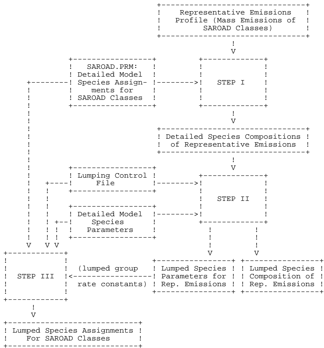
Figure 3. Diagram of the relationships between the three steps of the operation of the PREPEMIT program and data sets employed.
