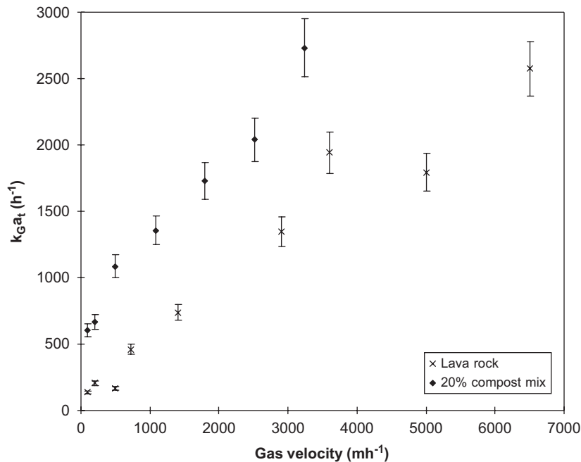
Fig. 9. Mass transfer coefficient ( k_G a_t ) of a lava rock bed compared to a 20% vol compost–woodchips mixture. Error bars indicate the experimental uncertainties.
