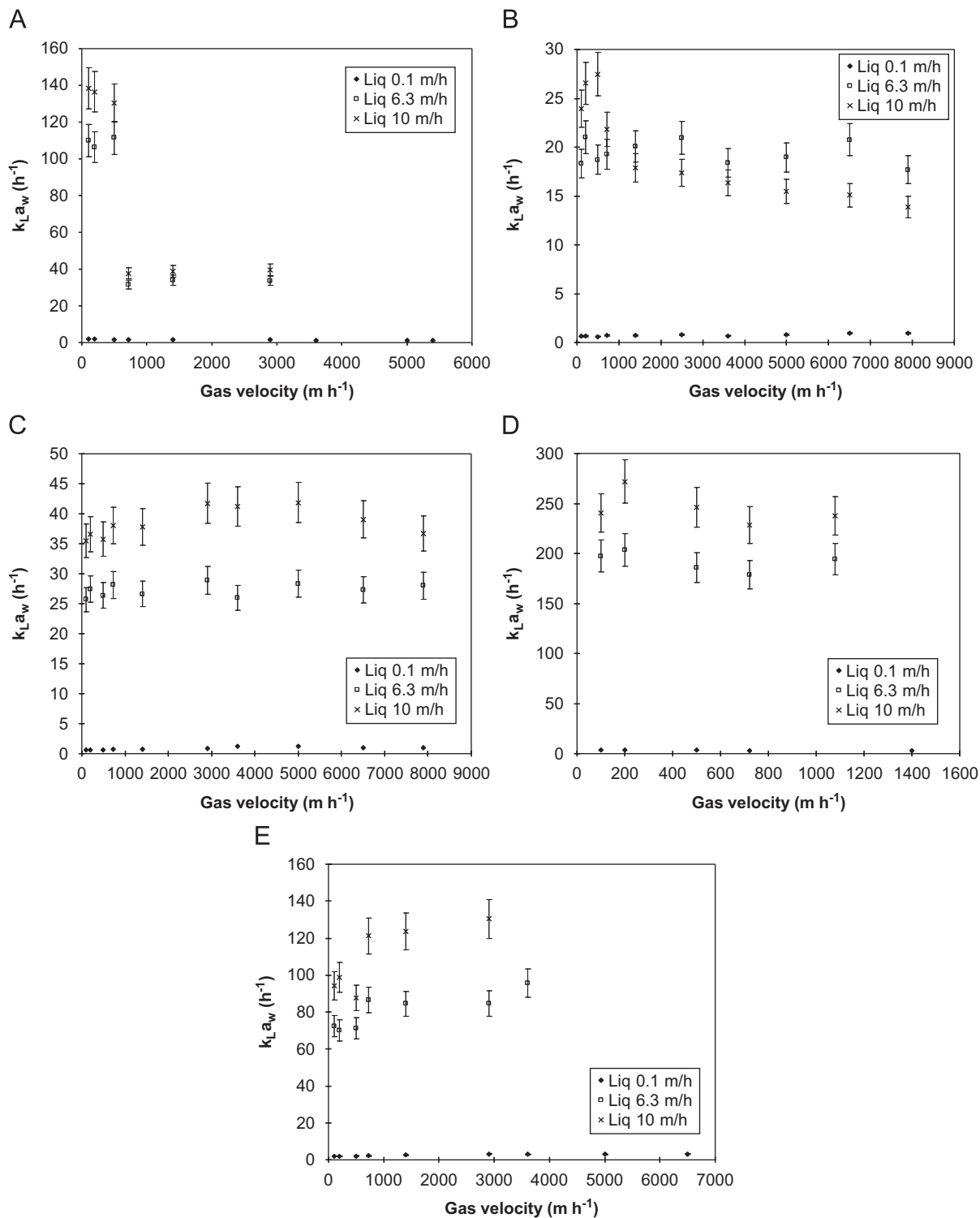
Fig. 16. Effect of gas velocity on liquid film mass transfer coefficient ( k_{La_w} ) in biotrickling filters. Packing materials: (A) lava rock, (B) PU foam, (C) 1 in Pall ring, (D) porous ceramic beads, (E) porous ceramic rings. Note the different y scales between the graphs. Error bars indicate the experimental uncertainties.
