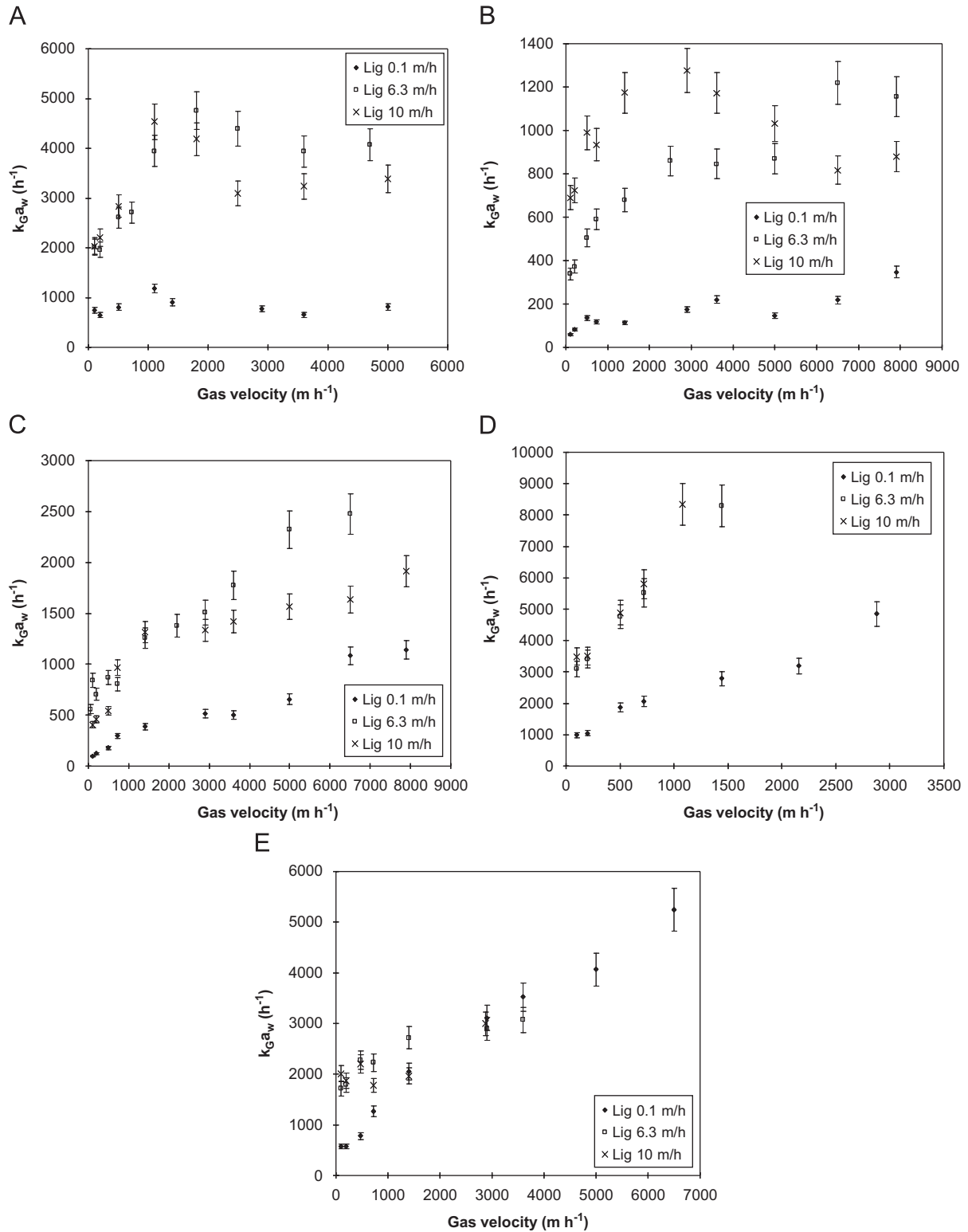
Fig. 12. Effect of gas velocity on gas film mass transfer coefficient ( k_G a_w ) in biotrickling filter. Packing materials: (A) lava rock, (B) PU foam, (C) 1 in Pall ring, (D) porous ceramic beads, (E) porous ceramic rings. Note the different x and y scales between the graphs. Error bars indicate the experimental uncertainties.
