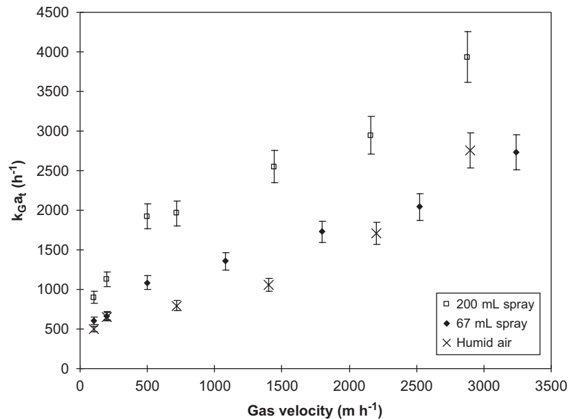
Fig. 3. Effect of moisture supply method on k_G a_t . Compost mixture with woodchips (20:80, v/v) was used as packed bed. Error bars indicate the experimental uncertainties.
