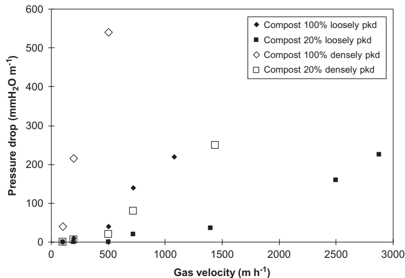
Fig. 6. Effect of packing nature and density on pressure drop.
