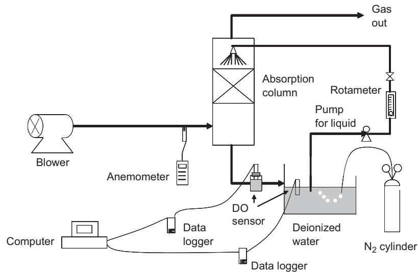
Fig. 2. Schematic of the experimental setup for k_L a_w .
