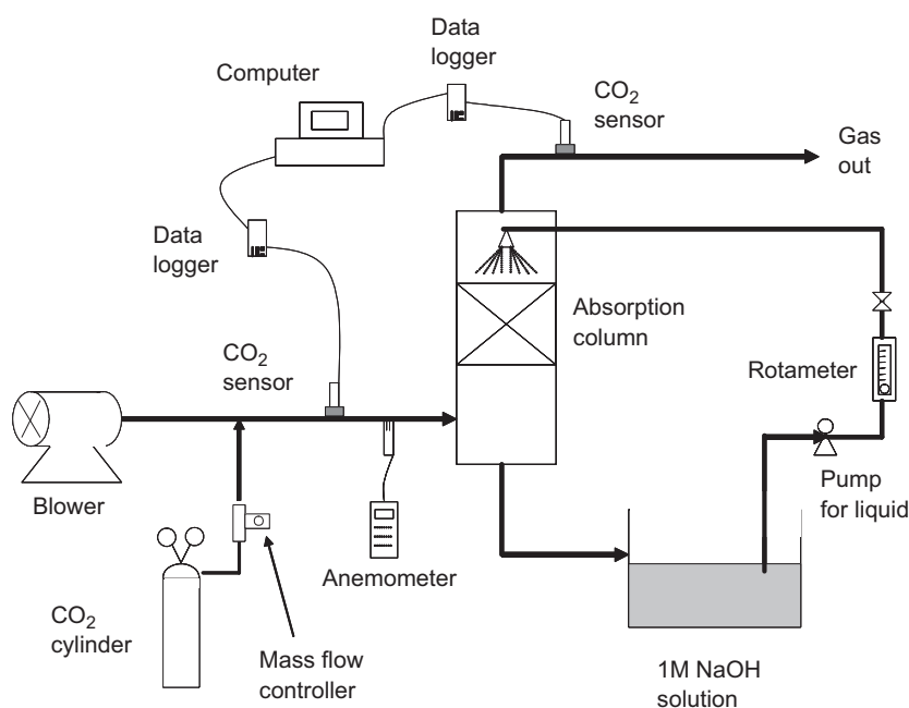
Fig. 1. Schematic of the experimental setup for k_{G a_w} .
