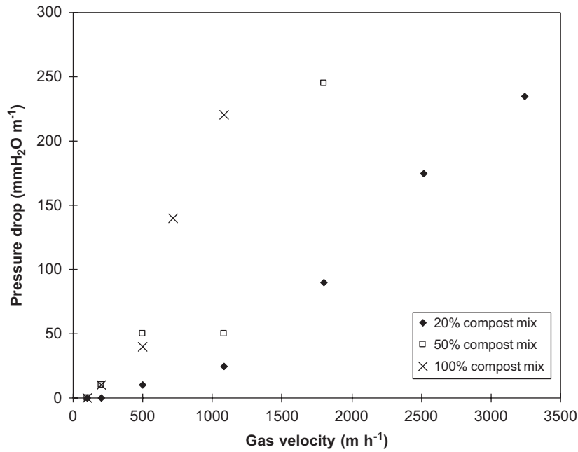
Fig. 8. Effect of compost and woodchips volume ratio on pressure drop.
