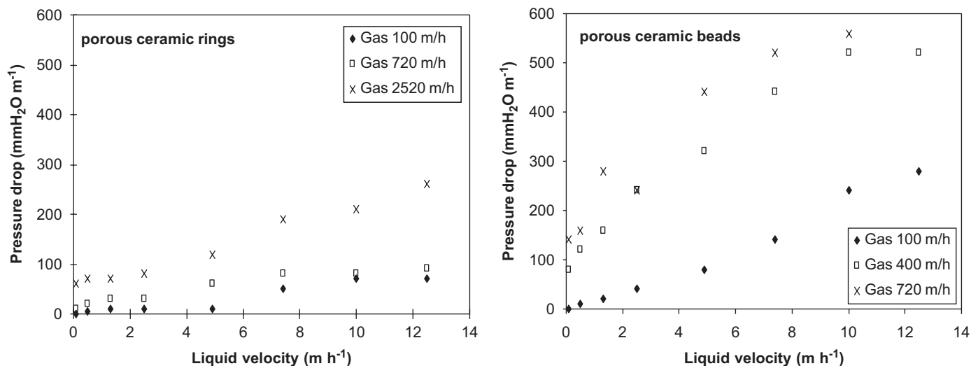
Fig. 15. Pressure drop during the mass transfer experiments for the porous ceramic rings (left) and beads (right).
