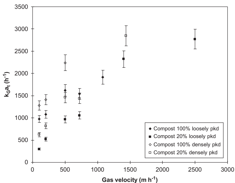
Fig. 5. Effect of packing nature (compost and woodchips mixtures) and density on gas film mass transfer coefficient ( k_{Ga_t} ). Loosely packed bed had a density of 220 \text{ kg m}^{-3} , while the densely packed density was 330 \text{ kg m}^{-3} . Error bars indicate the experimental uncertainties.
