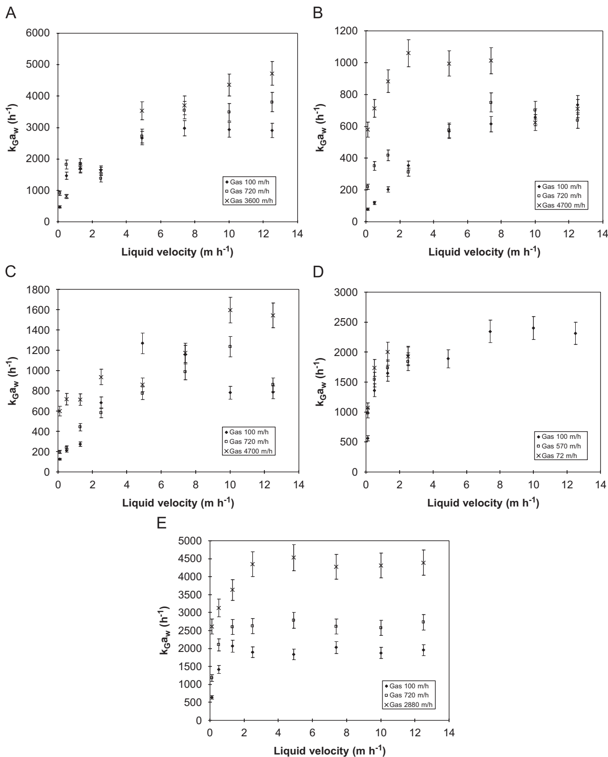
Fig. 13. Effect of liquid velocity on gas film mass transfer coefficient ( k_{Ga_w} ) in biotrickling filter. Packing materials: (A) lava rock, (B) PU foam, (C) 1 in Pall ring, (D) porous ceramic beads, (E) porous ceramic rings. Note the different y scales between the graphs. Error bars indicate the experimental uncertainties.
