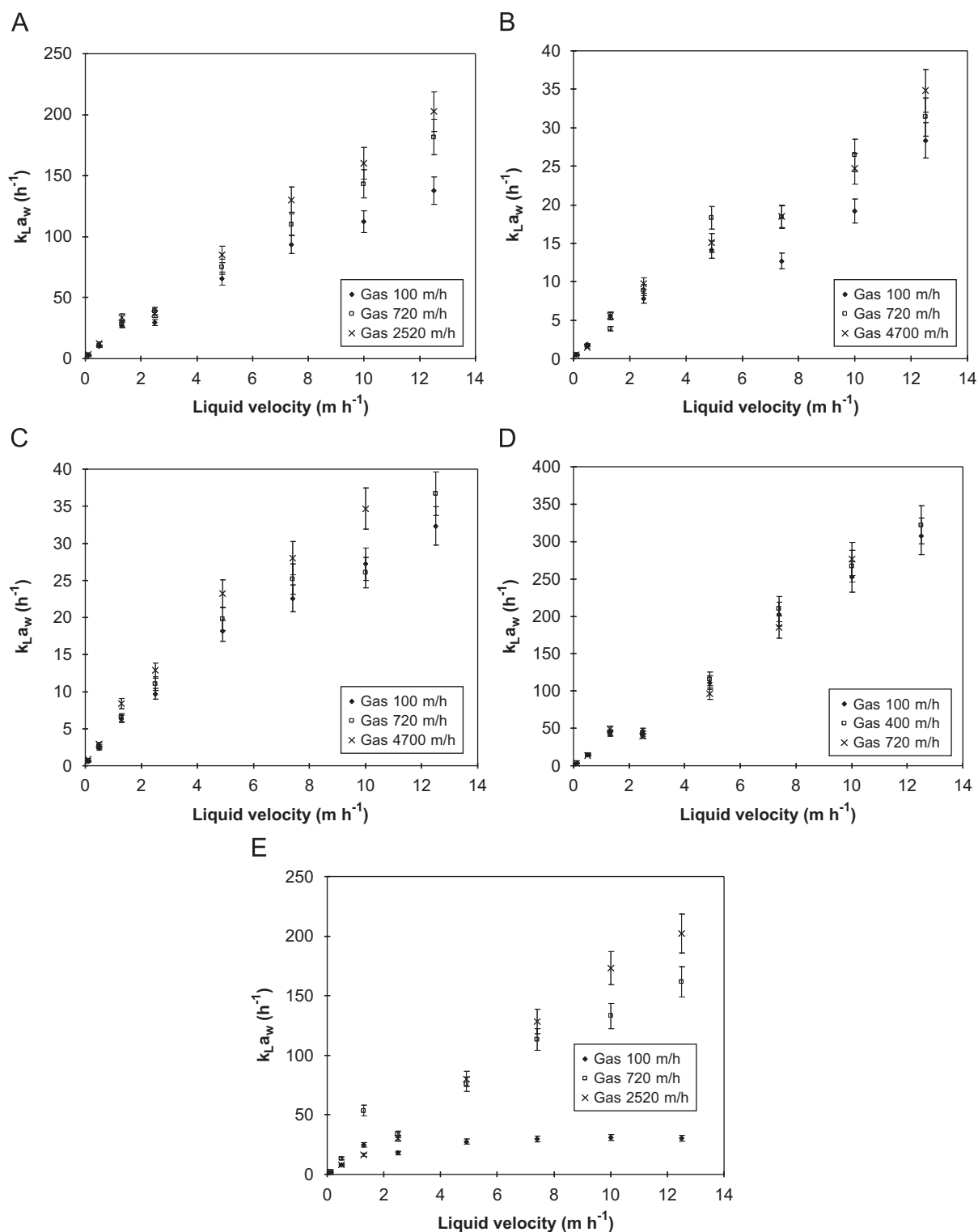
Fig. 14. Effect of liquid velocity on liquid film mass transfer coefficient ( k_L a_w ) in biotrickling filter. Packing materials: (A) lava rock, (B) PU foam, (C) 1 in Pall ring, (D) porous ceramic beads, (E) porous ceramic rings. Note the different y scales between the graphs. Error bars indicate the experimental uncertainties.
