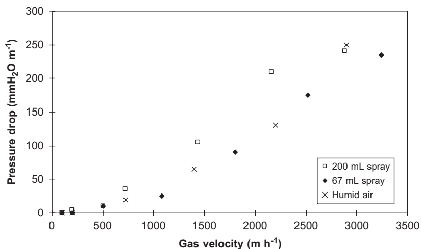
Fig. 4. Pressure drop over the 20:80% vol compost–woodchips bed for different moisture management methods.
