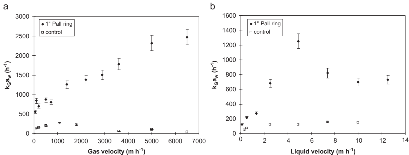
Fig. 11. Effect of gas velocity (a) and of liquid velocity (b) on mass transfer using 1 in Pall Ring compared to an empty column control. (a) Liquid linear velocity was 6.3 \text{ m h}^{-1} . (b) Gas linear velocity was 1000 \text{ m h}^{-1} . Error bars indicate the experimental uncertainties.
