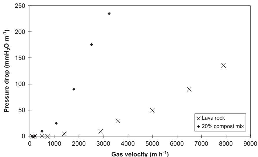
Fig. 10. Comparison of pressure drop of lava rock and compost-woodchips beds.
