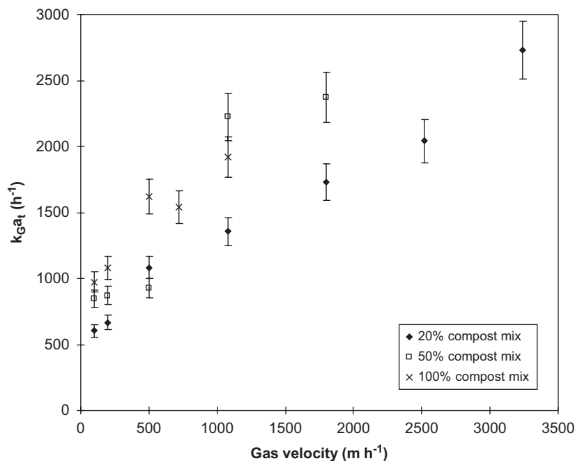
Fig. 7. Effect of compost and woodchips volume ratio on the mass transfer coefficient. Error bars indicate the experimental uncertainties.
