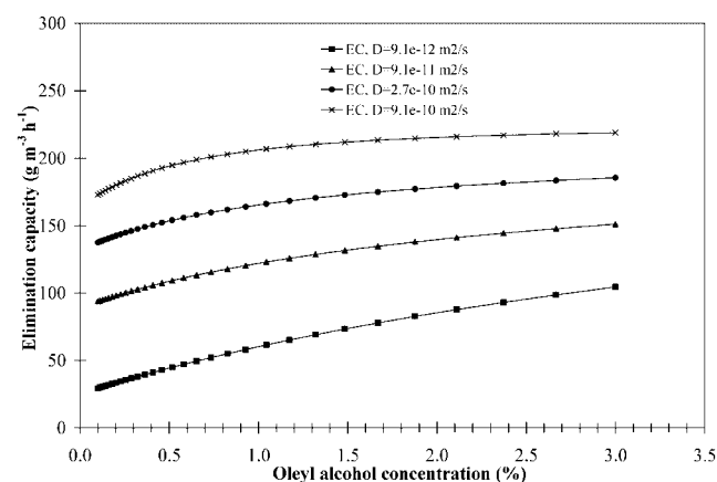
Figure 4. Model parametric sensitivity to oleyl alcohol concentration and the diffusion coefficient in the aqueous phase. Conditions for simulation: toluene inlet concentration, 1 \text{g m}^{-3} ; gas residence time, 15 s; biomass concentration, 16 \text{g}_{\text{dw}}\text{L}^{-1} ; FEBR height, 0.4 m.
